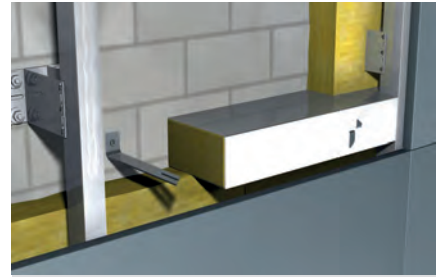
Installed FFB-VS Ventistop
